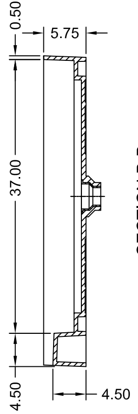
SECTION B-B
